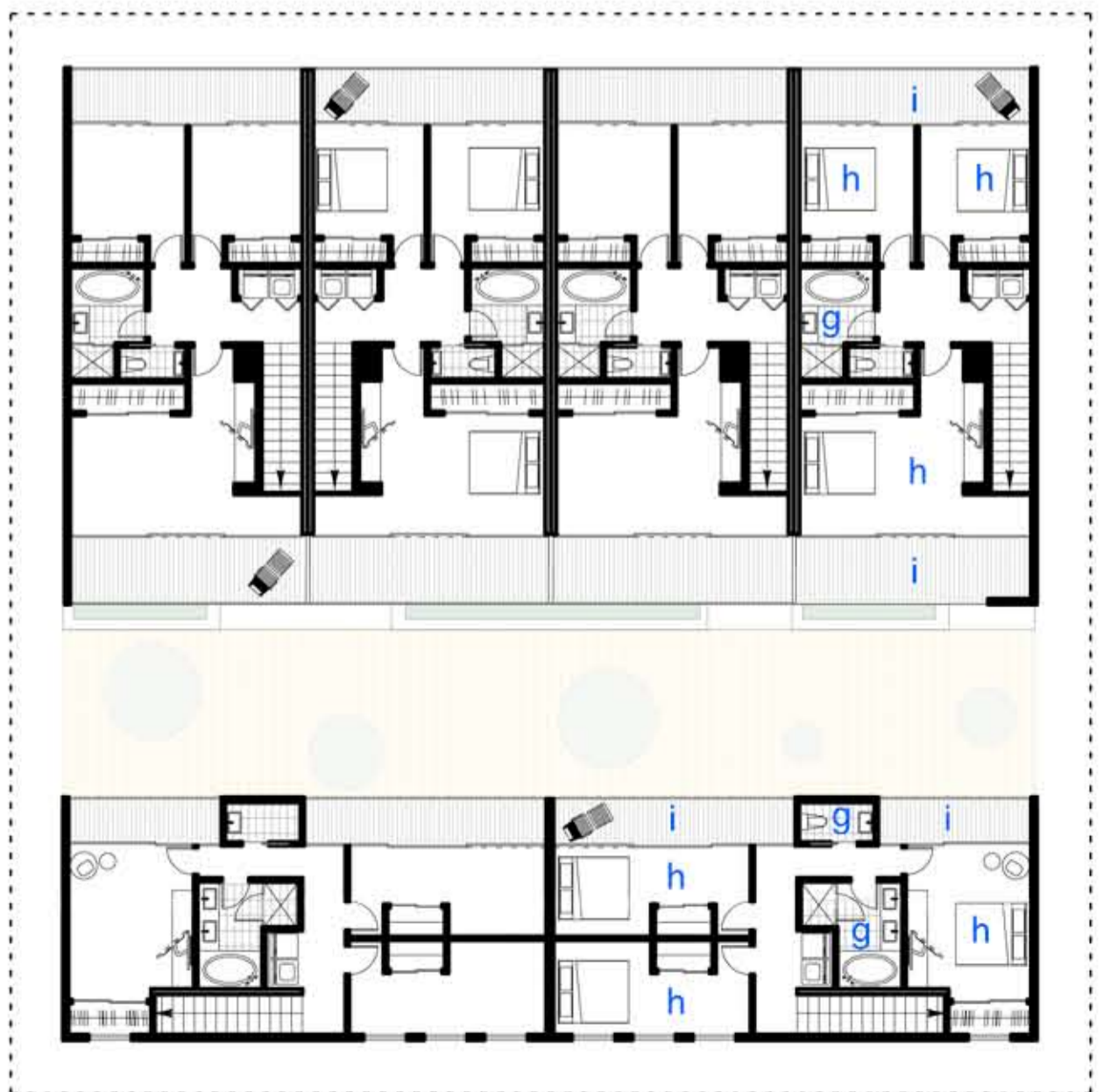
third floor
