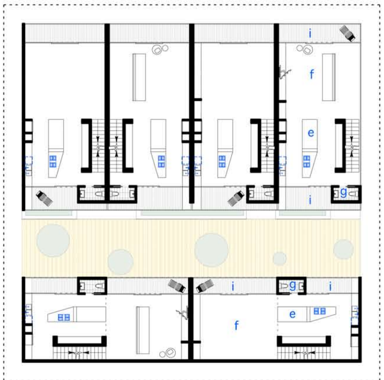
10' 25' 50' 1/16" = 1'
