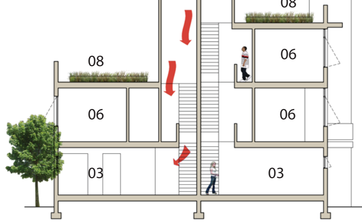
Section A 1/16" = 1'-0"
