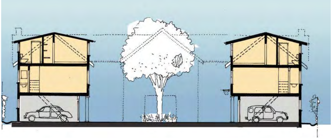
SECTION THROUGH COURTYARD Scale: 1/16"-1'-0"
