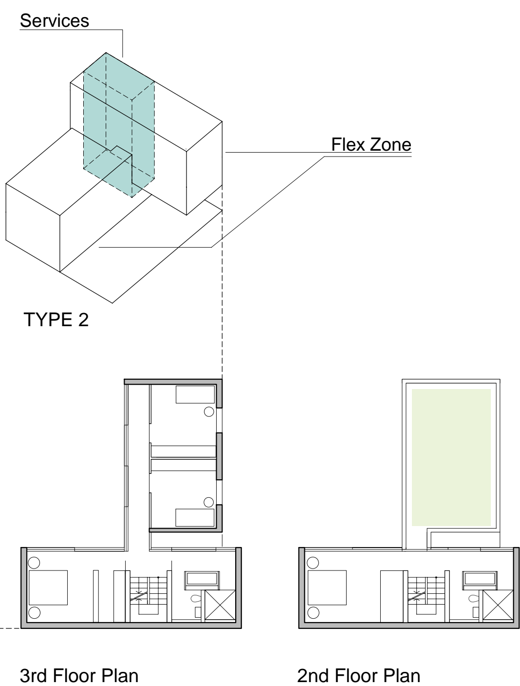
FLOOR PLANS - TYPE 2 Scale: 1/16"-1-0"
