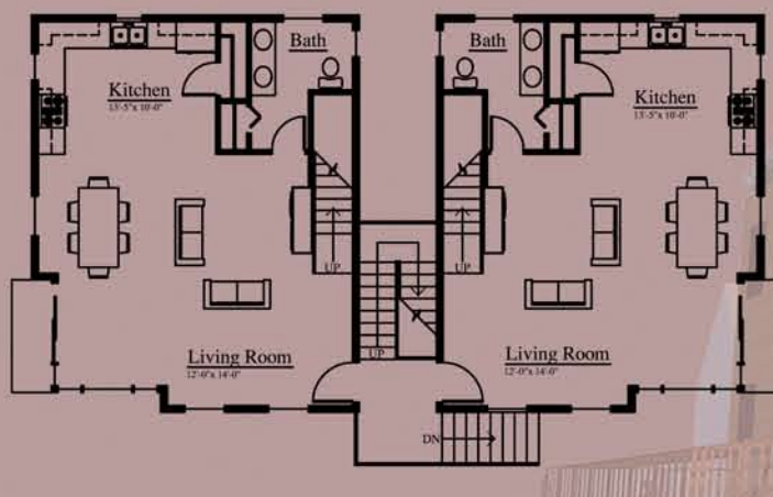
Unit B-First Floor Plan
