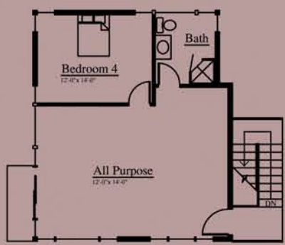
Unit A-Third Floor Plan
