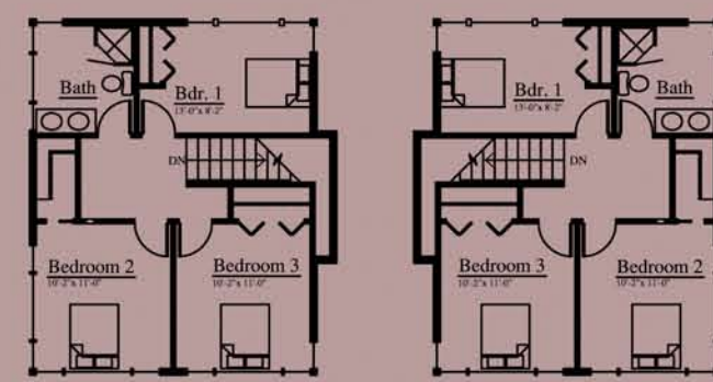
Unit C-Second Floor Plan
