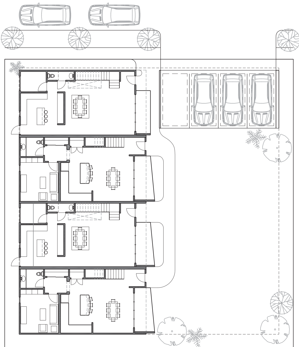
FIRST FLOOR / SITE PLAN
