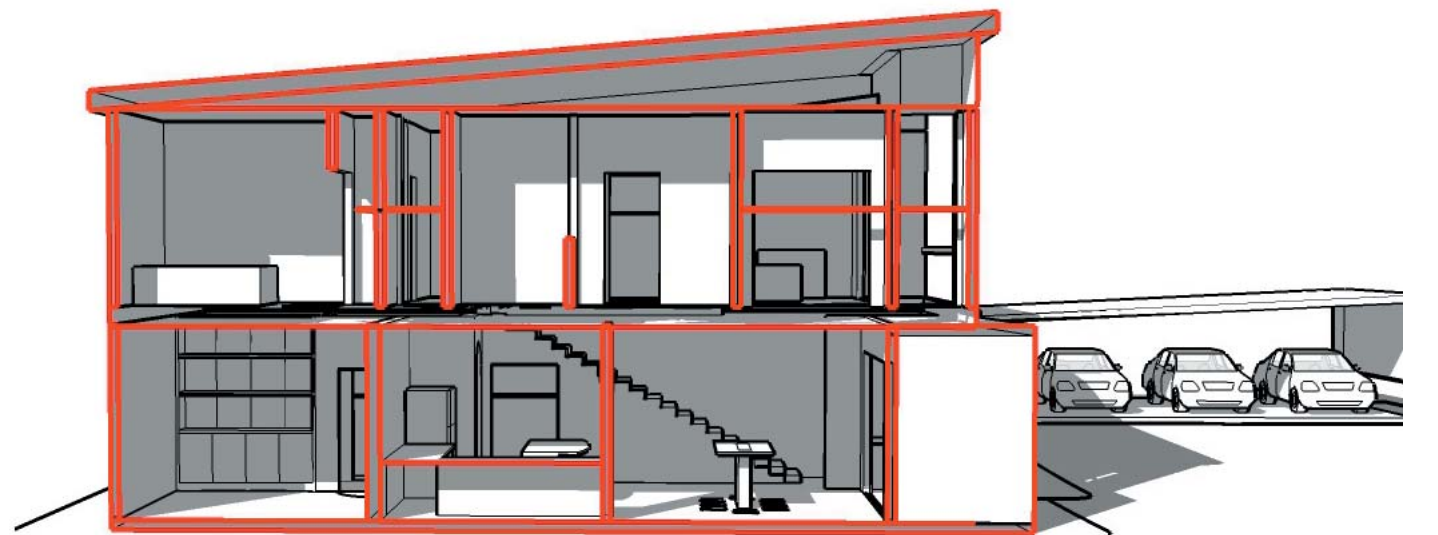
SOUTH UNIT SECTION
