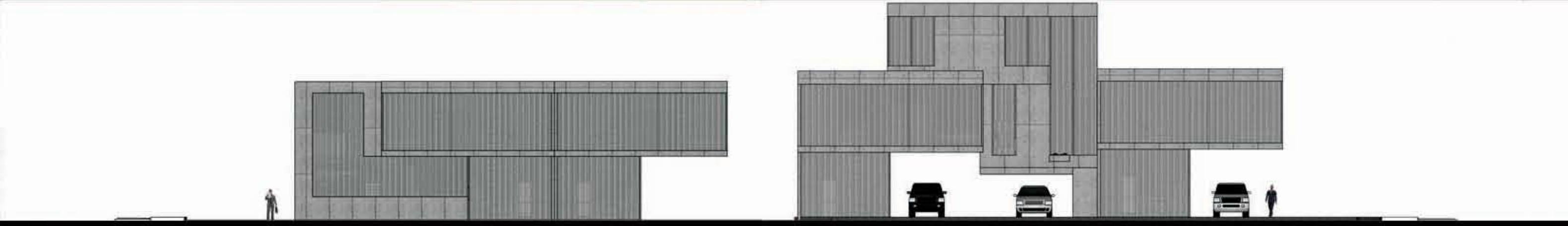
North Elevation North Unit
